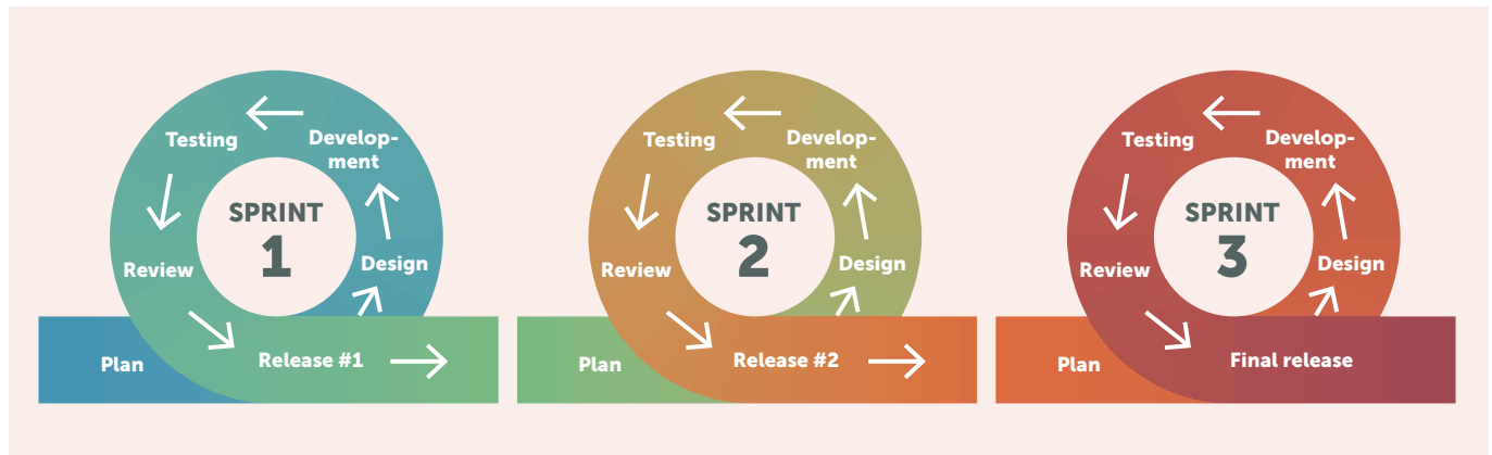
Figure 8. Agile methodology
